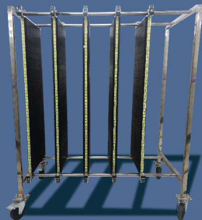
MAX PCB SIZE 400mm X 600mm
